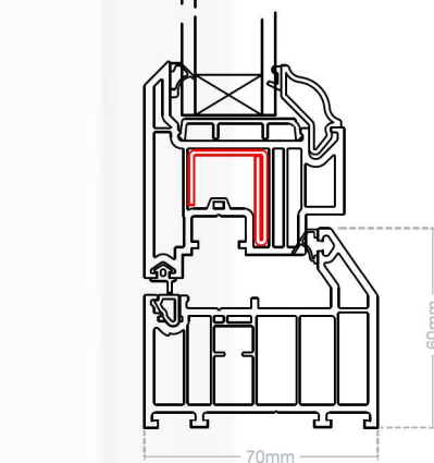
HORIZONTAL CROSS SECTION
