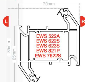
Intermediate transom Z EWS 7023
