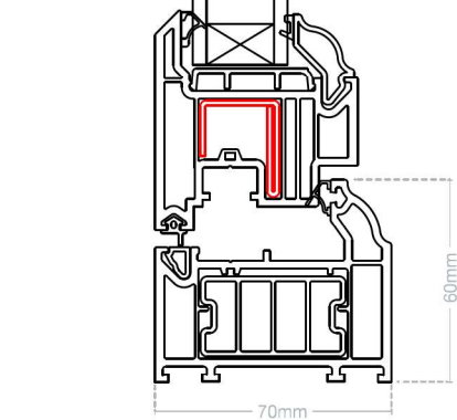
HORIZONTAL CROSS SECTION
