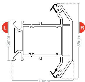
Intermediate transom T EWS 7022
