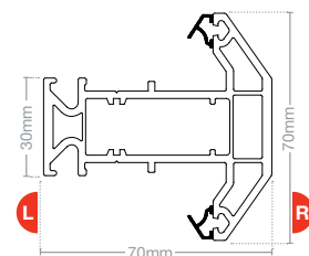
Transom T EWS 7002
